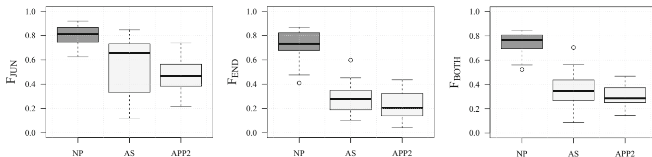
Fig. 19 Critical-point detection performance of our method (NP) compared to two other methods (AS and APP2). The median values of F_{JUN} (left plot) are 0.81 (NP), 0.65 (AS), and 0.47 (APP2). The
